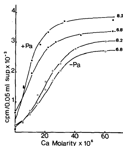
Fig.1. Competition for \text{Ca}^{2+} between myofibrils and parvalbumins, at pH 6.8 and pH 8.2. The displacement of ^{45}\text{Ca}^{2+} from the myofibrils into the supernatant is plotted in function of the quantity of cold \text{Ca}^{2+} added either under the form of \text{CaCl}_2 ( \circ, \square ) or as \text{Ca}_2 -parvalbumin ( \bullet, \blacksquare ). When the reasoning of Colowick and Womack [14] is applied to the first pair of curves ( \circ, \square ), dissociation constants of 0.66 \times 10^{-6} M and 0.52 \times 10^{-6} M can be calculated for 4.6 groups and 3.9 groups/mol myofibril, at pH 6.8 and pH 8.2, respectively. This conforms with the values found, in absence of \text{Mg}^{2+} , for the two \text{Ca}^{2+} -specific sites of troponin that are involved in the regulation of the myofibrillar ATPase activity [16]. The two sites with higher affinity were titrated too rapidly to permit the determination of their dissociation constant.
