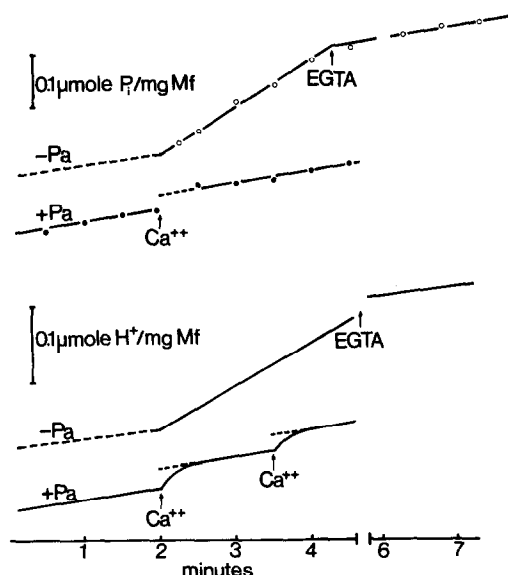
Fig. 2. Splitting of ATP by myofibrils initially in the \text{Ca}^{2+} -free state and subsequently activated by the addition of \text{CaCl}_2 . The production of hydrogen ions (—) or of \text{P}_i ( \circ, \bullet ) appearing in a 0.79/1.00 ratio, is reported in function of time, either in absence (— Pa) or in presence (+ Pa) of \text{Ca}^{2+} -free parvalbumin. In absence of \text{Ca}^{2+} -free parvalbumin, the levels of ATPase activity corresponding to the relaxed state were measured at the end of the experiments by addition of EGTA (final concentration 2 mM) and are reported as dotted lines at the start of the experiments.
